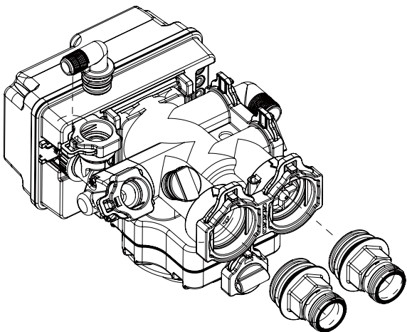
Description: Straight, Inlet/Outlet Size: Male 1", 1.25", 1.5" Type: QC, Thread, BSP/NPT Used on: 95
