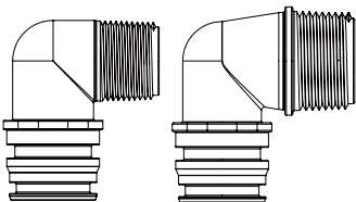
Description: Elbow, Drain Line Size: Male 3/4", 1" Type: QC, Thread, BSP/NPT Used on: 89/95
