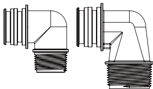
Description: Elbow, Inlet/Outlet Size: Male 1", 1.25" Type: QC, Thread, BSP/NPT Used on: 89
