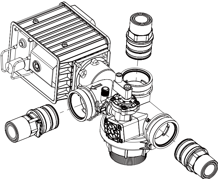
Description: Straight, Drain Line Size: Male 1.5", 2" Type: QC, Thread, BSP/NPT Used on: 105
